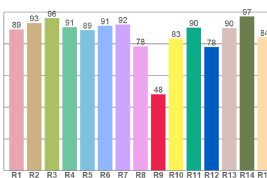
CRI: 90.0 (R1-R8)
